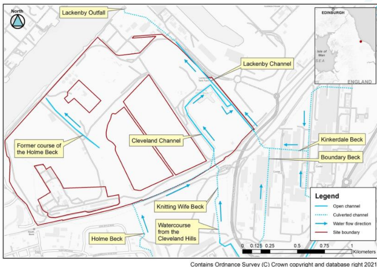
Figure A-1: Site boundary and watercourses through and surrounding the site
