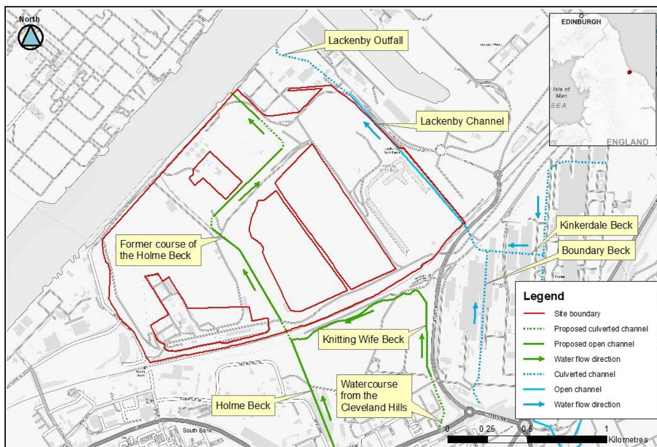
Figure 3-2: Proposals for watercourses on site
