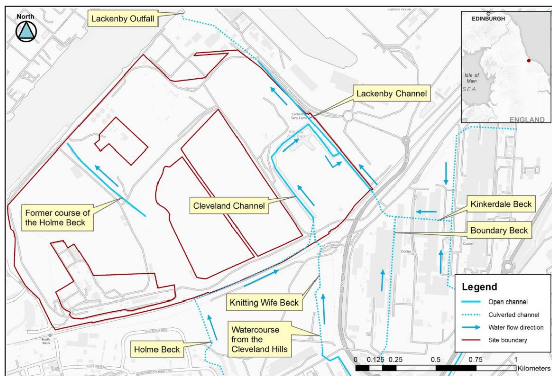
Figure B- 1: Site boundary and watercourses through and surrounding the site
